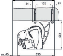
Top-fix
